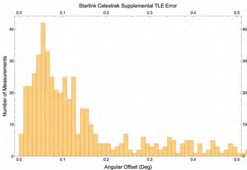
Figure D.2.5. The majority of TLE predictions are less than 0.2 degrees off from the actual satellite position. Large errors are present and extend all the way to >0.5 degrees, the limit of the telescope’s FOV and thus ability to measure.
