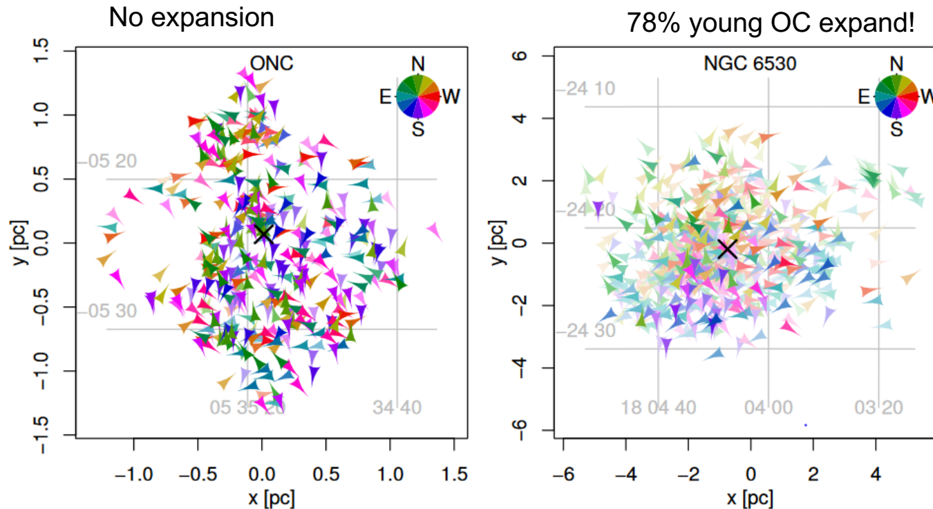
Figure 3. Direction of motion of individual stars in the rest frame of the cluster. Diagrams are shown for the ONC (left) and NGC 6530 (right). The orientations of the arrows and their hues indicate their direction, while saturation indicates weighting based on statistical uncertainty. In the ONC stars with different velocities are mixed together, while, in NGC 6530, many stars have directions of motions away from the cluster center (as indicated by the outward pointing arrows and color segregation by azimuth). Plots for other clusters are included in an online figure set.
