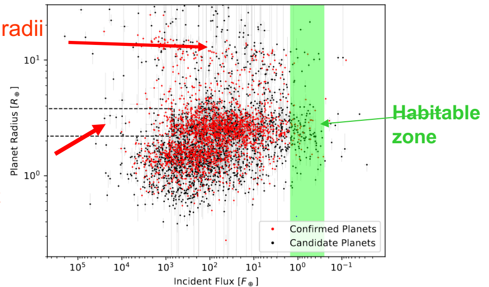
Figure 9. Planet radius versus incident flux for Kepler exoplanets. Red and black dots are confirmed and candidate exoplanets, respectively. We also plot our asymmetric error bars in transparent gray. The dashed line box represents the extension of the super-Earth desert identified in Lundkvist et al. (2016), while the green bar indicates the approximate optimistic habitable zone for FGK stars as detailed in Kane et al. (2016).
