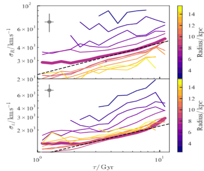
Figure 10. Velocity dispersions against age for a series of radial bins (for giant and turn-off stars with |z| < 0.6 kpc and [M/H] > -1 dex). Each line is coloured by the mean Galactocentric radius of the bin. The top panel shows
