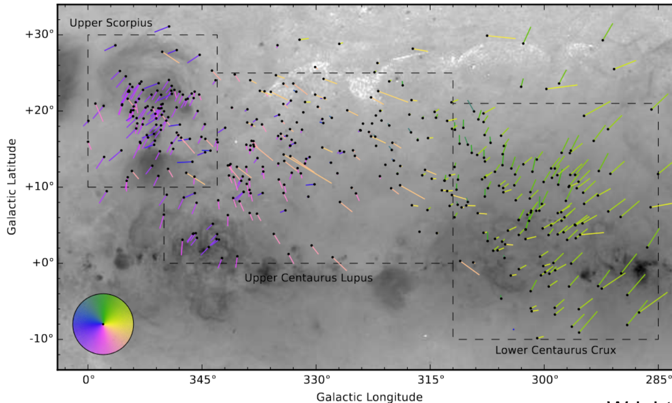
Figure 12. Proper motion vector map for the entire Sco-Cen association projected onto an inverted H \alpha image from Finkbeiner (2003) . The proper motions were corrected for radial streaming motion according to the equations in Brown et al (1997) and using bulk (median) RVs of -6.2, 2.8 and 13.0 km/s for the three subgroups. Points show the current positions of stars and vectors show the proper motions over 0.5 Myr with the bulk (median) proper motion of the entire association subtracted to show the relative motion. The vectors have been colour based on their direction of motion (see colour wheel in lower-left) to highlight kinematic substructure.
