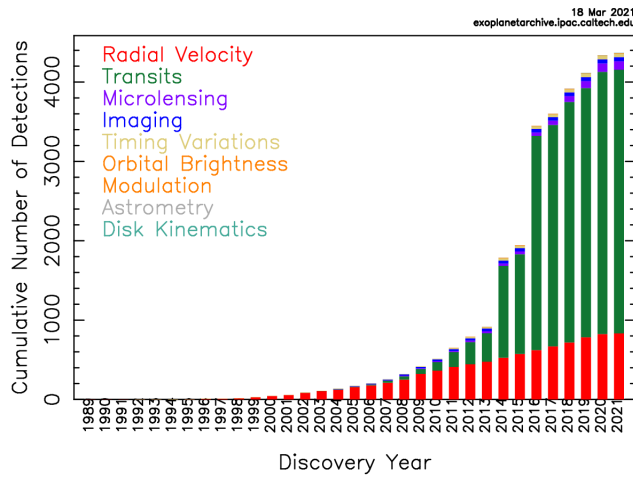
Figure 4. Cumulative number of exoplanet detections per year by different discovery methods (Plot taken from NASA Exoplanet Archive https://exoplanetarchive.ipac.caltech.edu/ )
